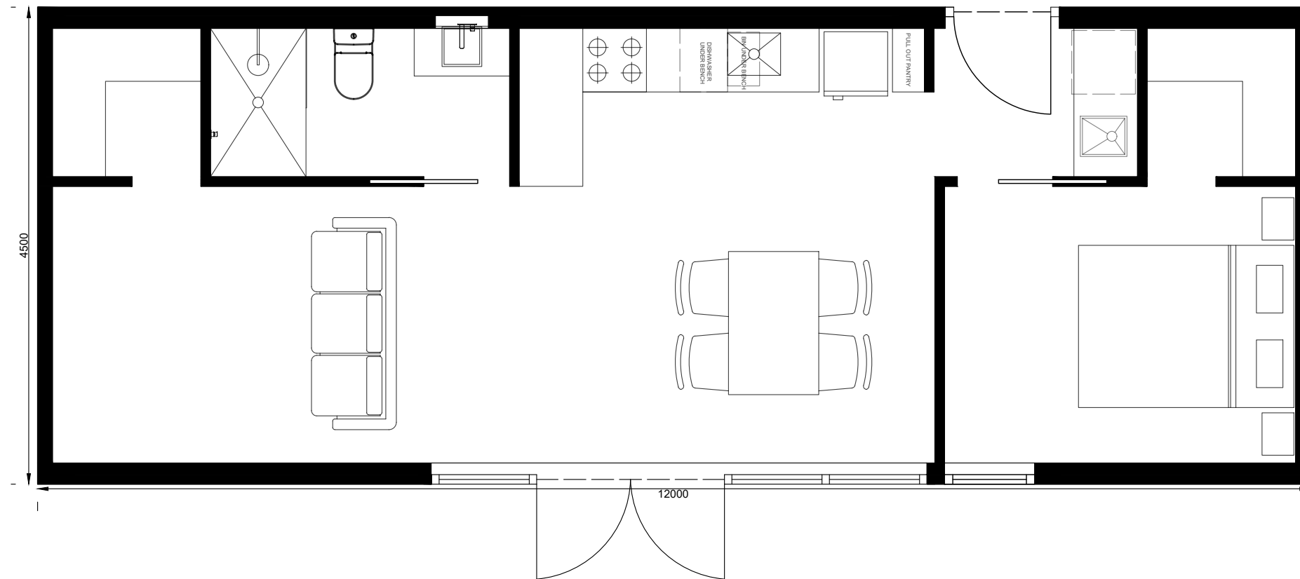
1-2-BEDROOM FLOOR PLAN
